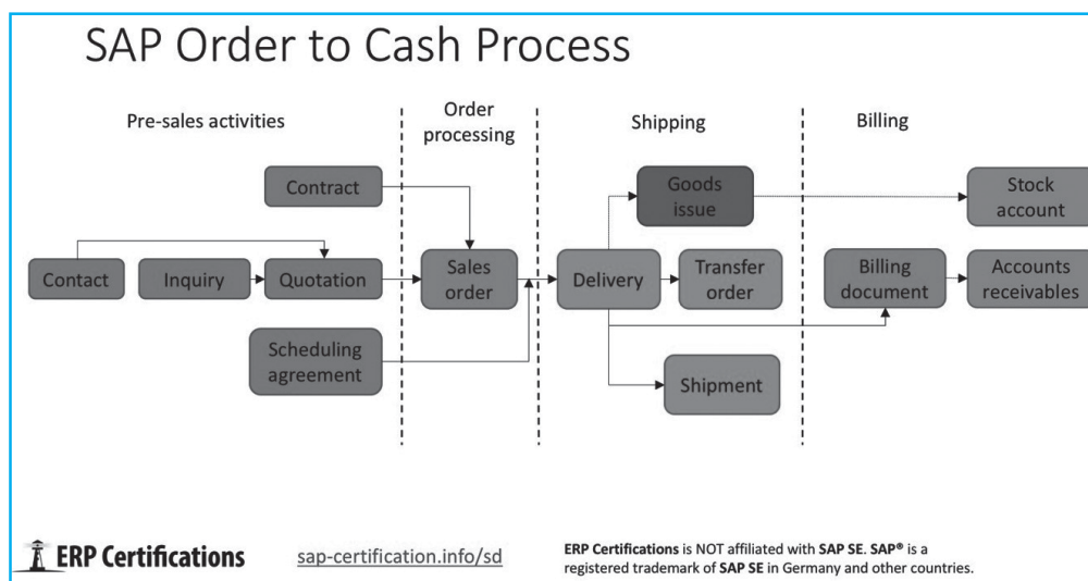
Figure 2.5: Order-to-Cash Process
